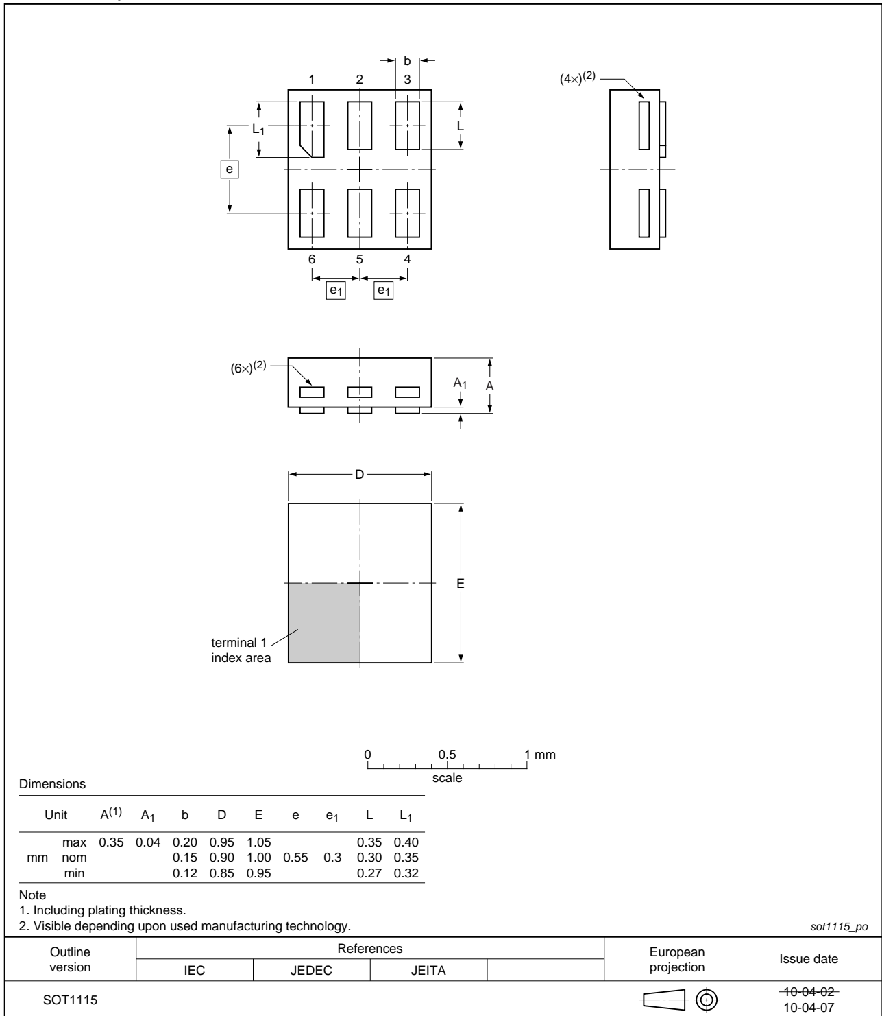
Fig 20. Package outline SOT1115 (XSON6)
